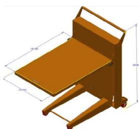
Pick-up cart
